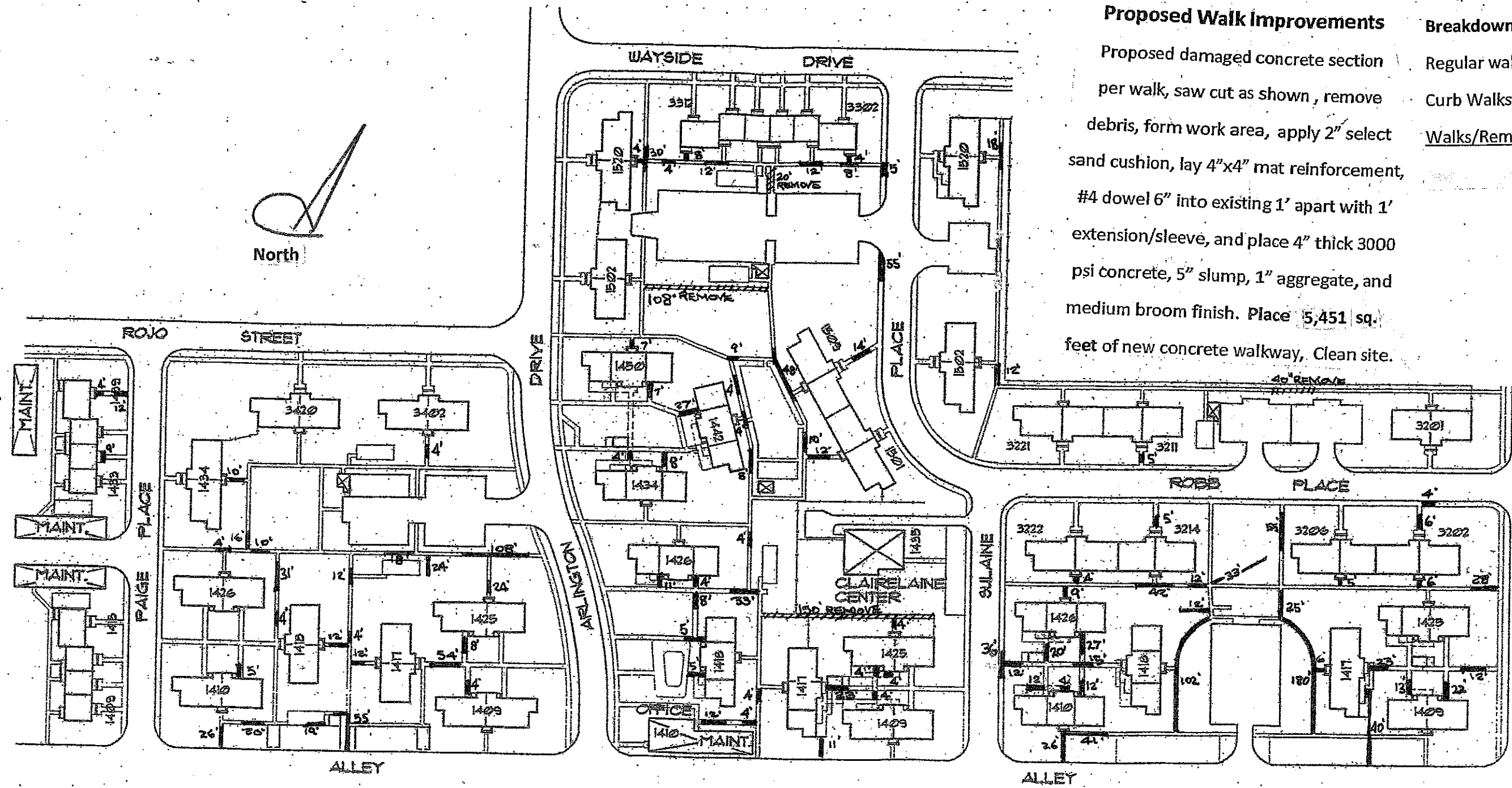
Clairelaine Gardens Proposed Walk Improvements N.T.S.
